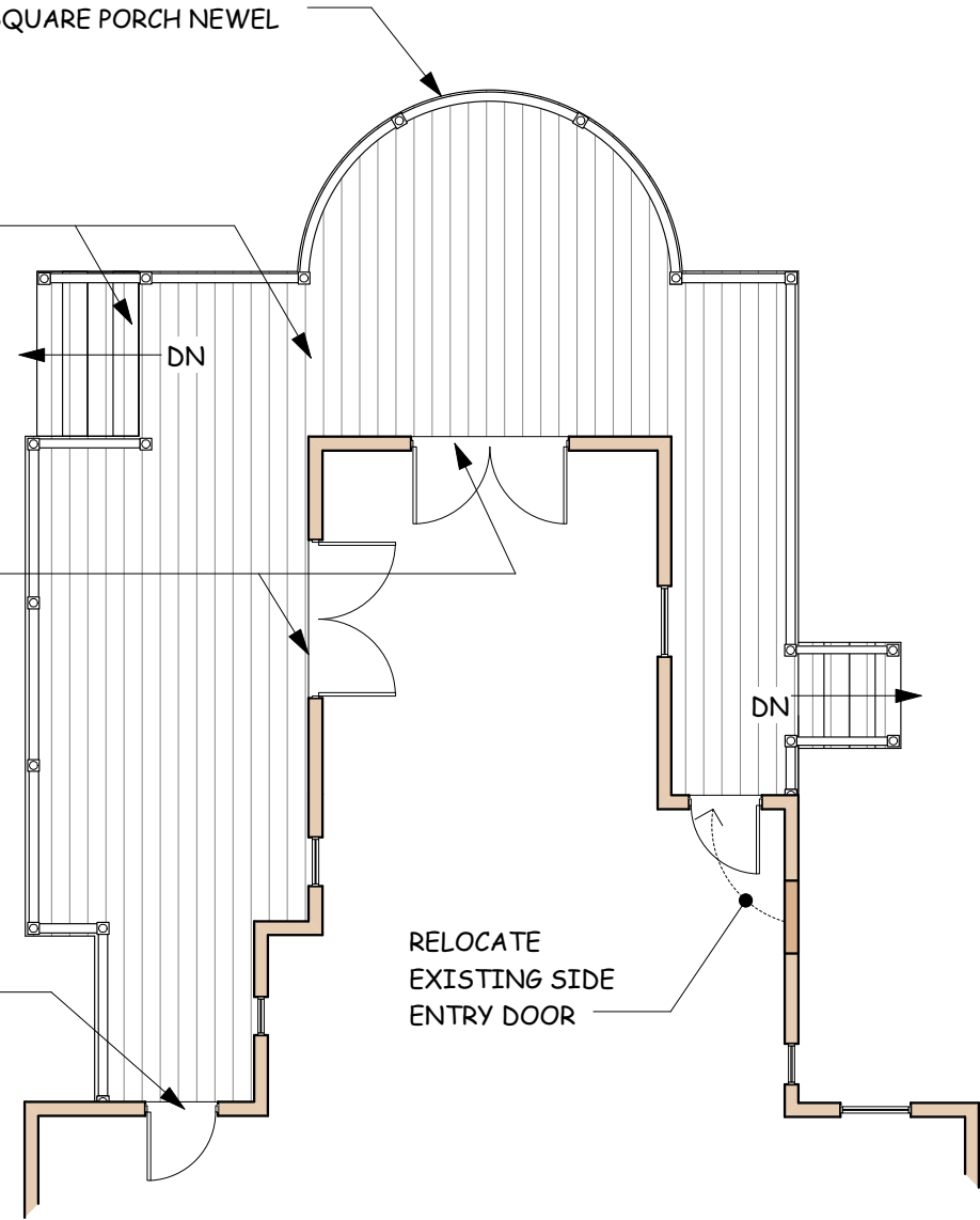
PROPOSED DECK PLAN
